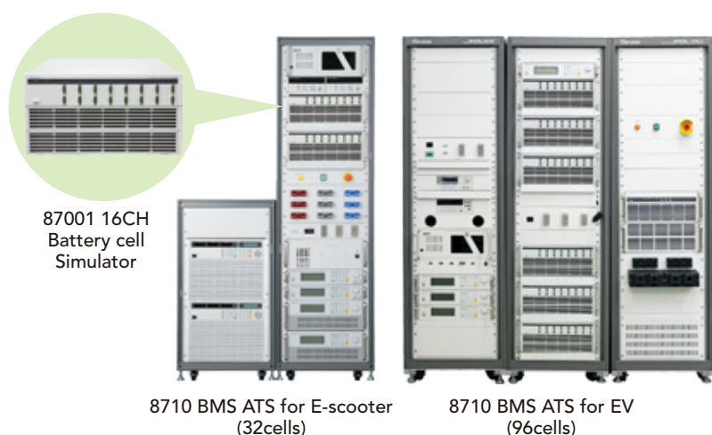
BMS Test System 8710 & Battery Cell Simulator 87001
