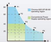
Constant Power Wide Range
