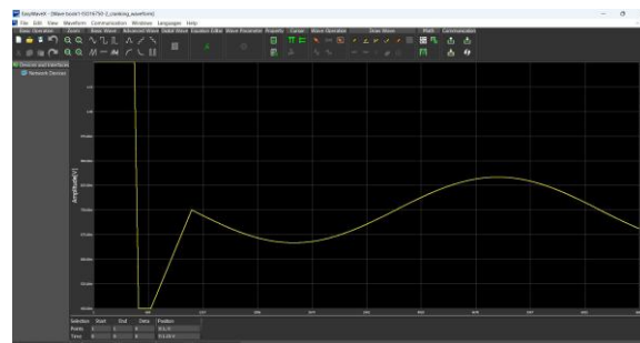
Figure 3: ISO16750-2_cranking_waveform.csv, zoomed section
