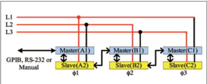
Figure 12: Parallel/3-Phase Delta connection
