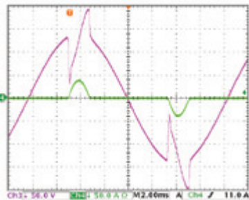
Figure 9: With ABA
