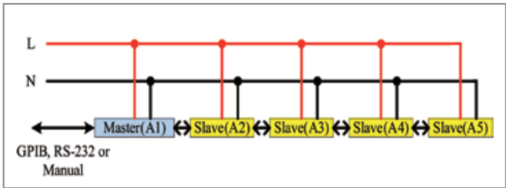
Figure 10: Parallel connection
