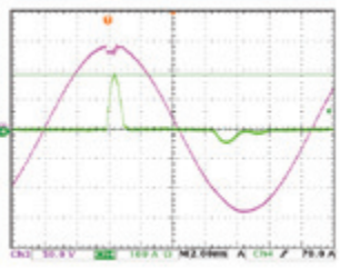
Figure 6: Inrush Current Mode
