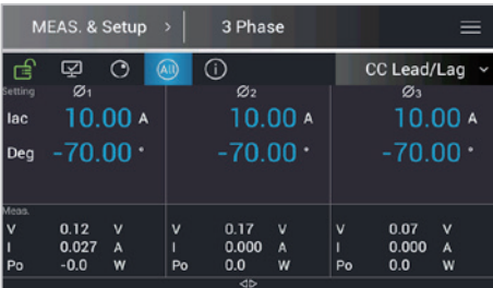
CC Lead/Lag Mode (Three-Phase)
