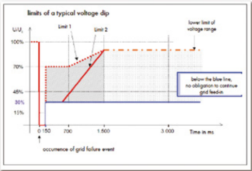
LVRT Test Curve
