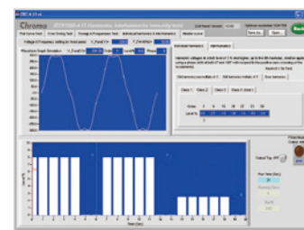
Voltage Harmonic & Interharmonics Test
